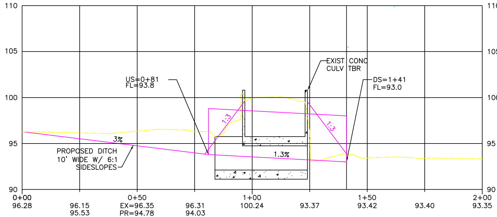
STREAM PROFILE (60° SKEW TO ROADWAY CENTERLINE)
